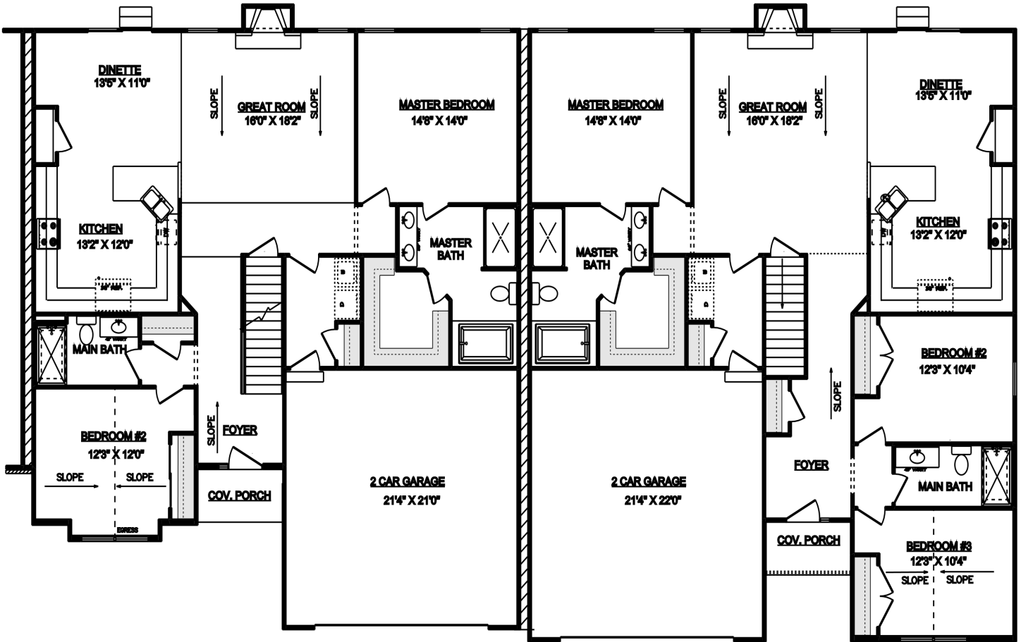
UNIT 23 - FIRST FLOOR PLAN
